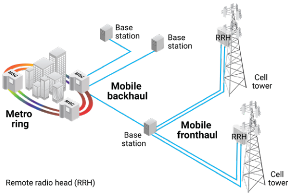
Figure 2. Backhaul mobile.
