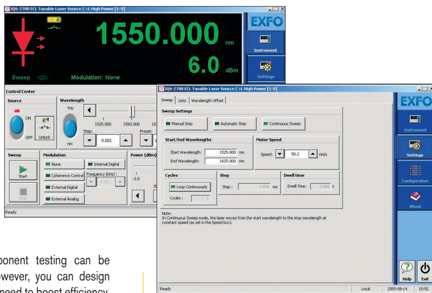
The IQS-2700's main user interface and sweep menu.
