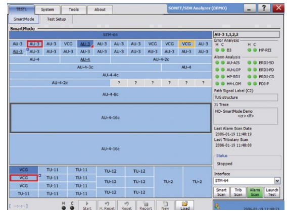
IQS-8130NGE SmartMode: multichannel signal discovery with real-time alarm scan.
