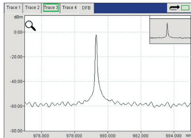
External cavity 980 nm laser spectrum showing high resolution and sharp response.
