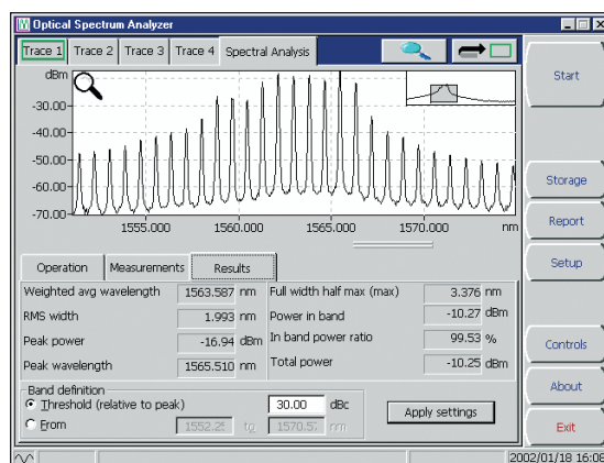
Automatic calculation of most common spectral characteristics. Above—a calculation based on power underneath the trace.
