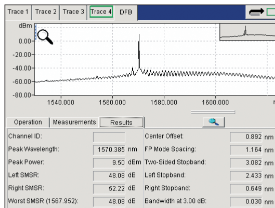
Analysis of the DFB signal acquired in trace 4. The Measurements tab gives access to functions such as power between markers. Eleven parameters can be measured. Results can be saved as an ASCII file or retrieved through the GPIB bus or using ActiveX commands.
