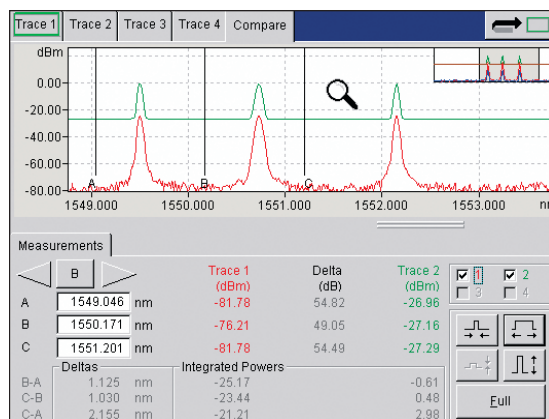
The Compare function allows you to display up to 4 traces. Two traces can be compared using markers for integrated power, power levels and more.
