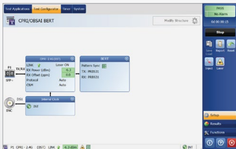
Figure 7. Framed CPRI BER Test
