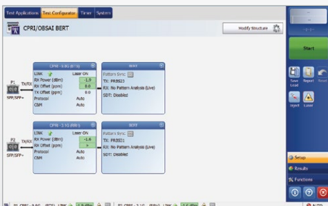
Figure 8. Dual Port CPRI BER test
