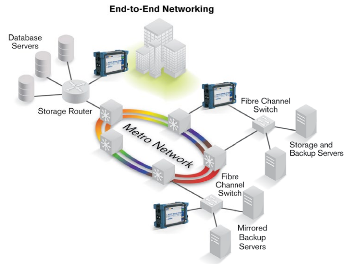
Figure 10. Thanks to end-to-end network testing capabilities, EXFO's Power Blazer enables fast deployment and configuration of FC networks. Communication between the transport network, interconnection devices and end nodes can be validated with features such as BER testing, latency measurement, buffer-to-buffer credit estimation and port login capabilities.
