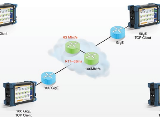
Figure 5. Baseline round-trip time (RTT) and bandwidth to determine ideal window size
