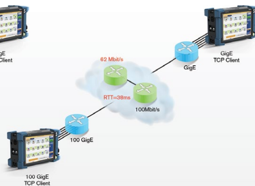
Figure 6. Single or multiple TCP connections to enable full pipe testing
