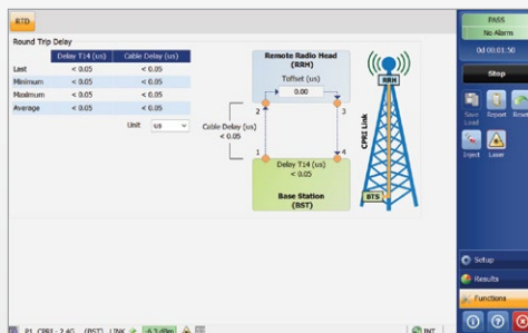
Figure 9. CPRI Round-Trip Delay
